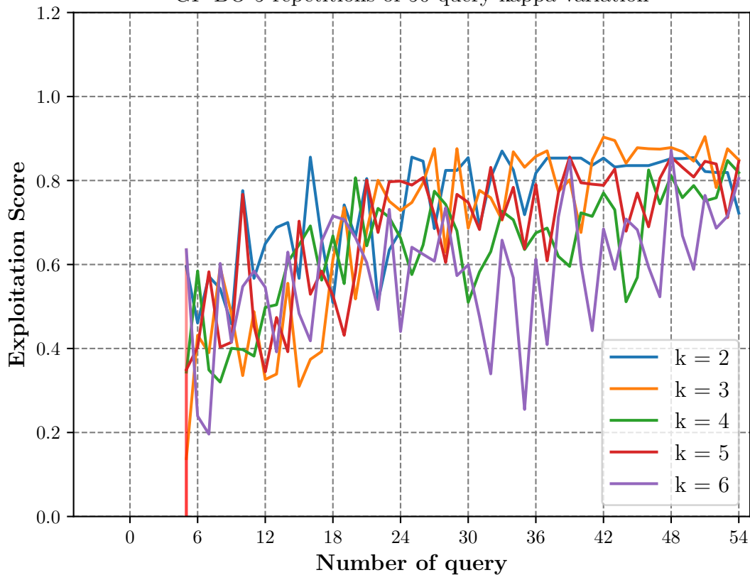
GP-BO 5 repetitions of 50 query kappa variation
